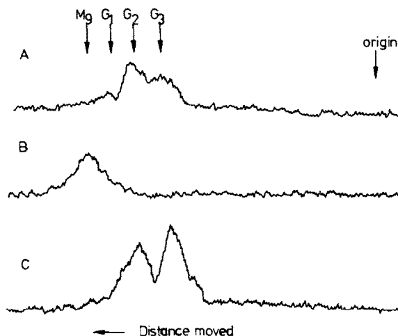
Fig.4. Chromatography of lipid-linked [ Glc\text{-}^{14}C ] oligosaccharide fraction from spinach. Microsomal fraction from spinach was incubated either with UDP-Glc (A) or GDP-Man (B) and the oligosaccharides released from lipid-oligosaccharide fraction was separated in solvent (B) as in fig.3. (C) is the Glc -oligosaccharide fraction from yeast.
