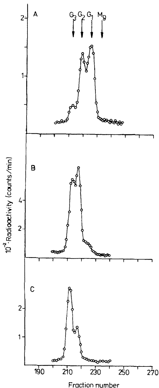
Fig.2. Gel filtration profile of [Glc-^{14}C] oligosaccharides from tobacco. Lipid-linked oligosaccharides were synthesized with UDP-Glc. The oligosaccharides were released from the chloroform/methanol/water (10/10/3, by vol.) extract by mild acid, treated with endo- N -acetylglucosaminidase and fractionated on Bio-Gel P4. (A) The profile of tobacco cells, (B) of yeast and (C) of liver synthesized according [13]. The arrows indicate the position of marker oligosaccharides M_9 , Man_9 , GlcNAc_1 , G_1 , G_2 , G_3 , Glc_{1,2,3} , Man_9 , GlcNAc_1 .
